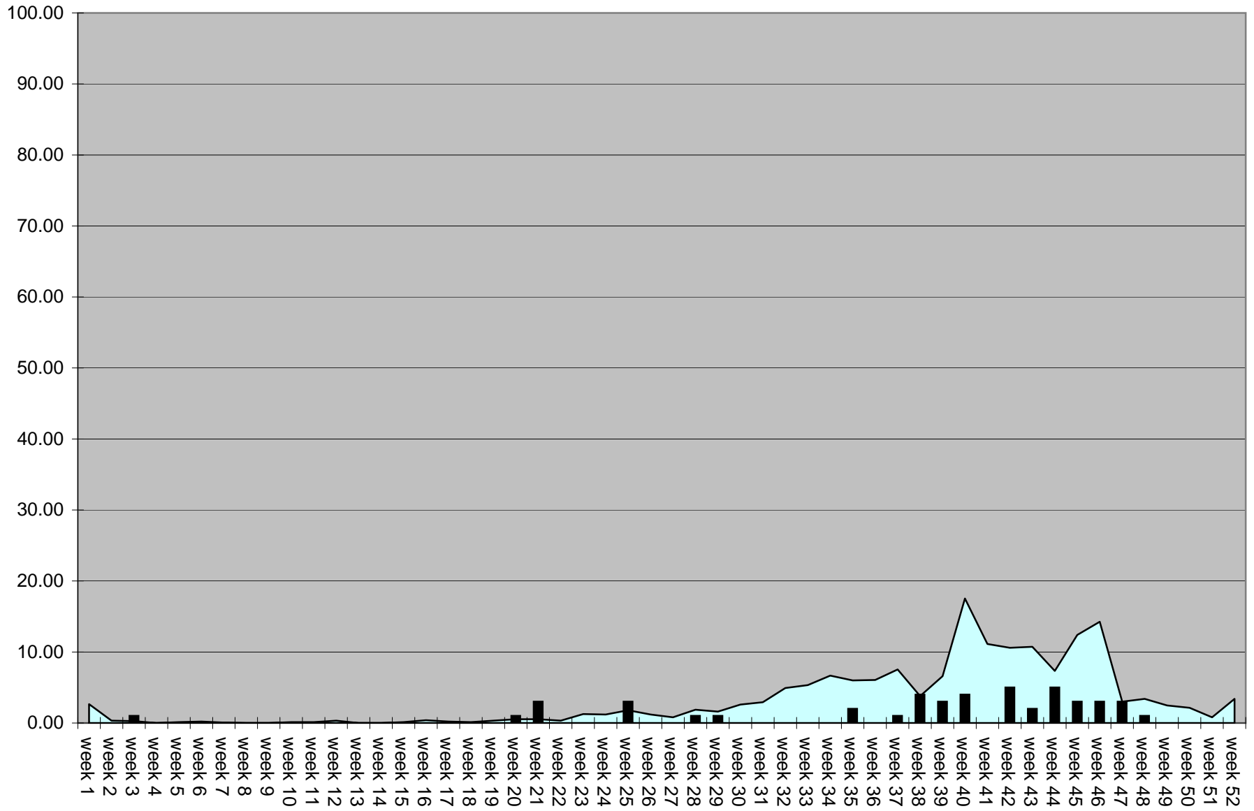
Culex pipiens complex Average ■ Cx. pipiens complex 2003
